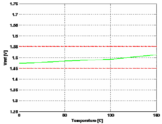
Error Amplifier V_{REF} vs. Junction Temperature
