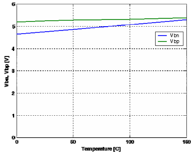
VBN & VBP (wrt VDD480) vs. Junction Temperature
