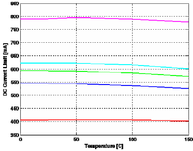
DC Current Limit vs. Junction Temperature 1
