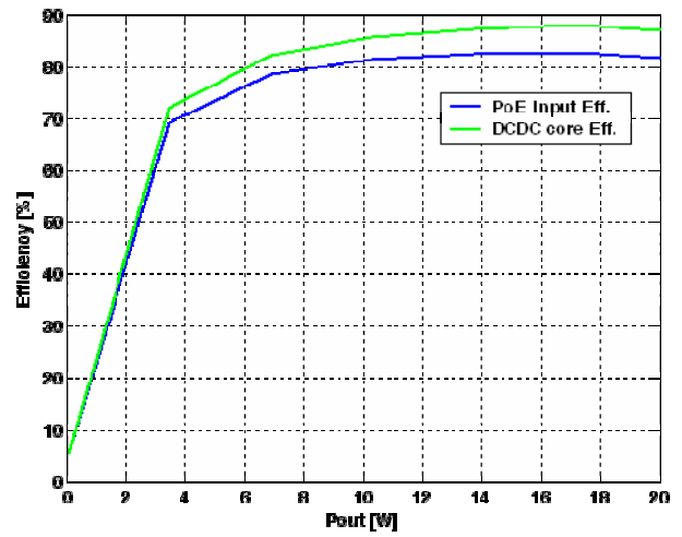
DCDC Efficiency vs. P_{OUT} @ V_{IN}=48V
