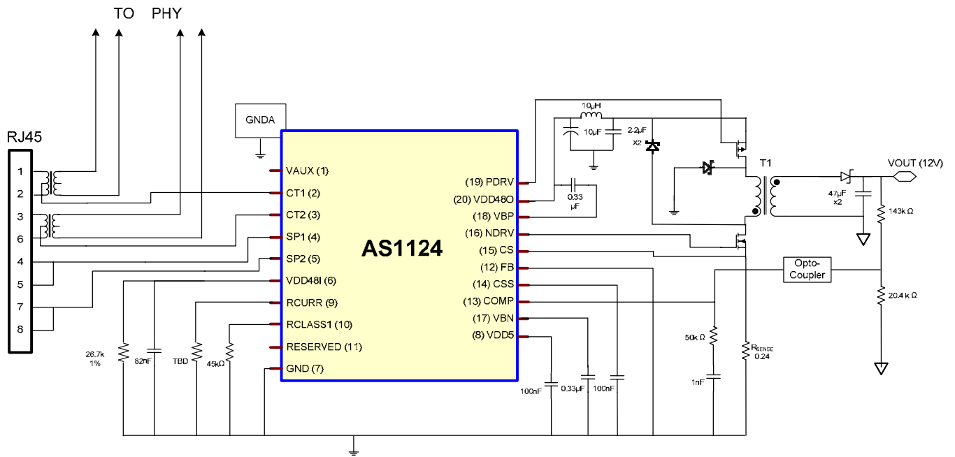
FIGURE 5. 10/100M WITH FLYBACK DC-DC CONVERTER
