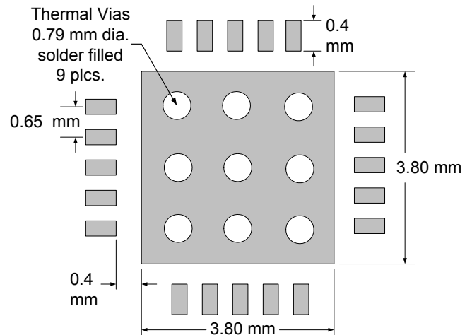
Figure 6. AS1124 PCB Footprint
