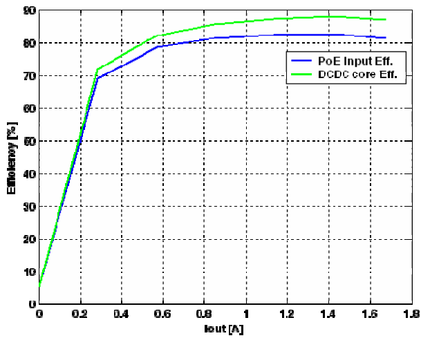
DCDC Efficiency vs. I_{OUT} @ V_{IN}=48V, V_O = 12V
