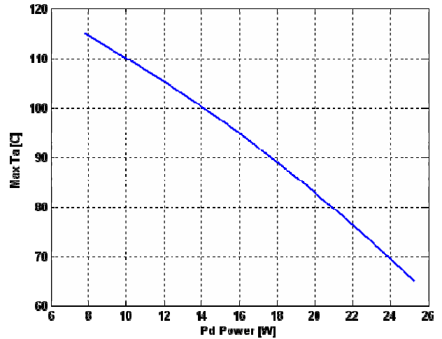
Figure 5. Thermal de-rating for high power operation
