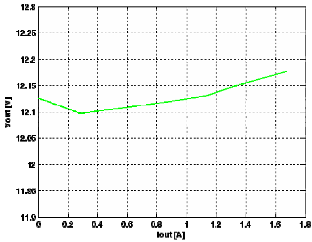
DCDC Load Regulation vs. I_{OUT} @ V_{IN}=48V, V_O = 12V
