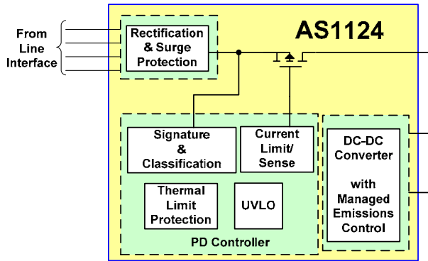
Figure 3. Top-Level Block Diagram of the AS1124
