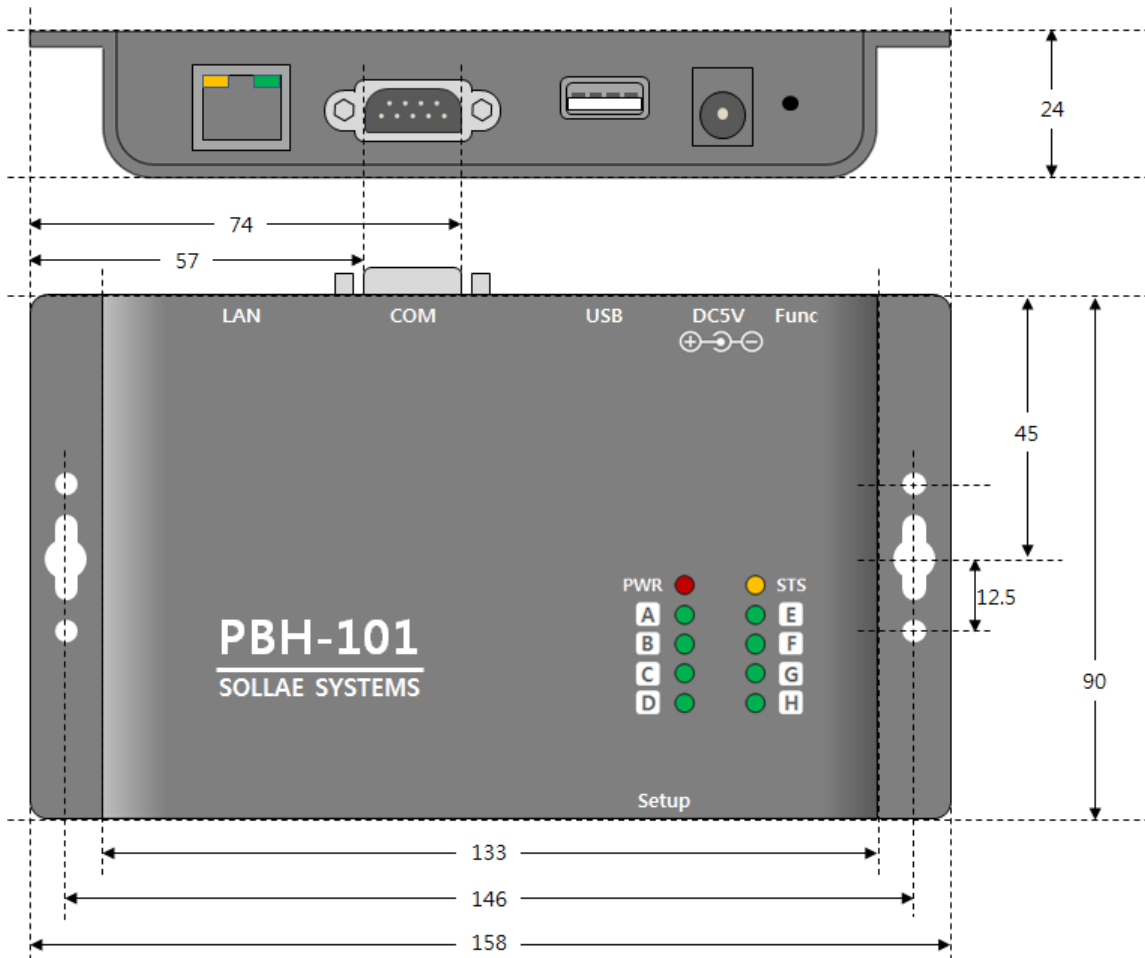
Figure 1-1 dimension
