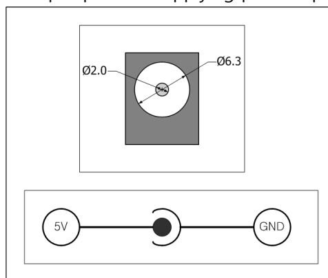
Figure 1-3 specification of power port
