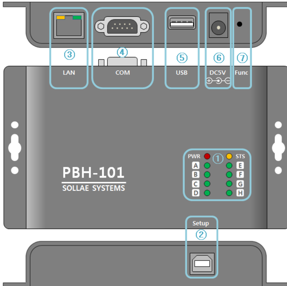
Figure 1-2 panel layout
