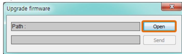
Figure 3-7 firmware upgrade (2)
