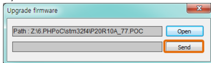
Figure 3-8 firmware upgrade (3)
