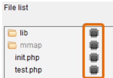
Figure 2-17 upload files
