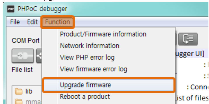
Figure 3-6 firmware upgrade (1)
