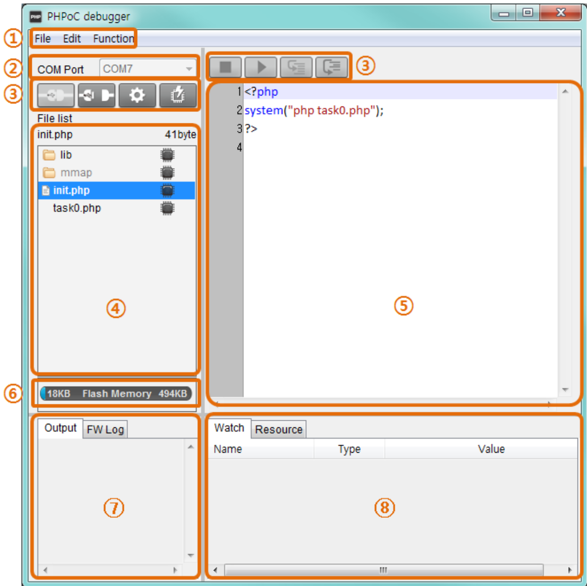
Figure 1-5 program structure
